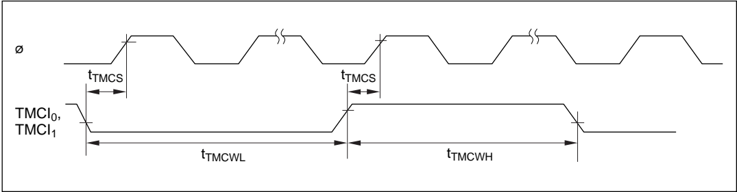
Figure 16-13 8-Bit Timer Clock Input Timing
