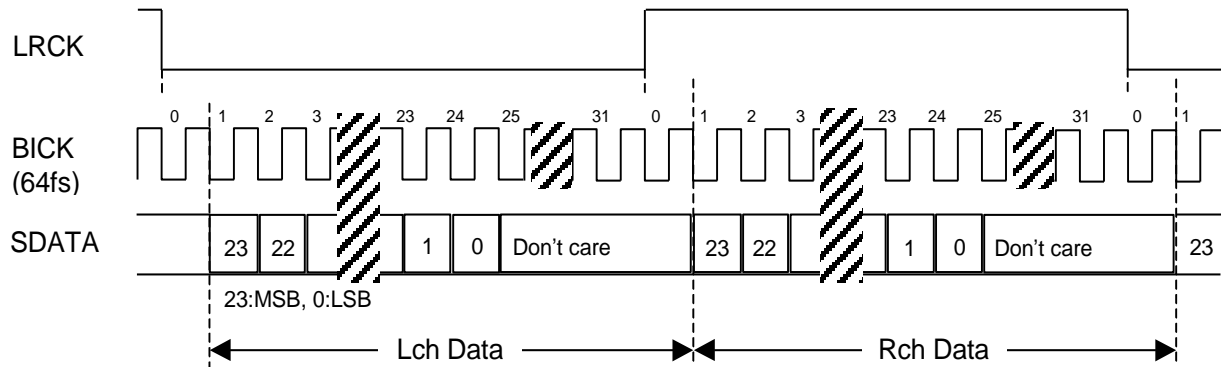
Figure 12. Mode 3 Timing
