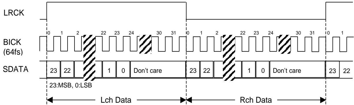
Figure 11. Mode 2 Timing
