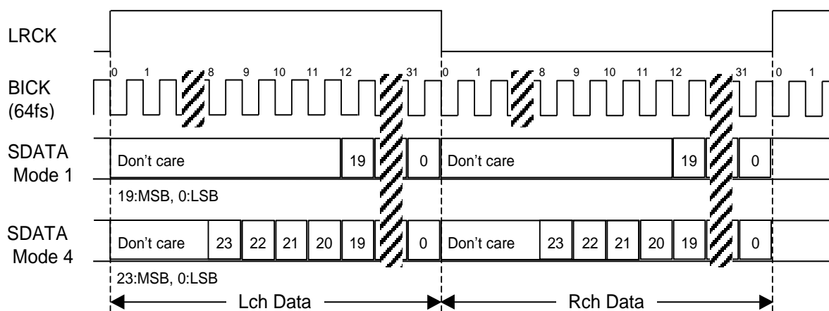
Figure 10. Mode 1/4 Timing
