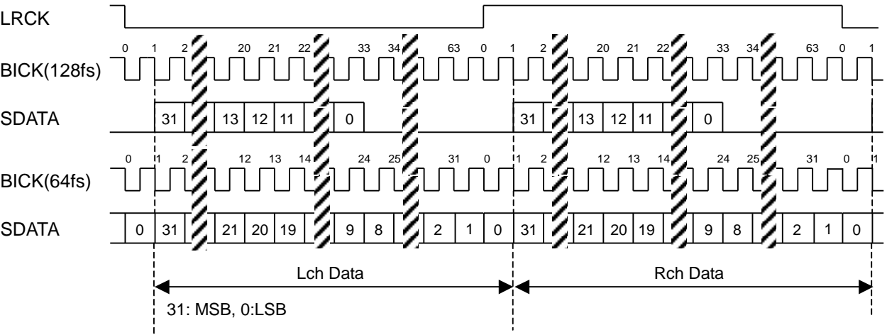
Figure 15. Mode 7 Timing
