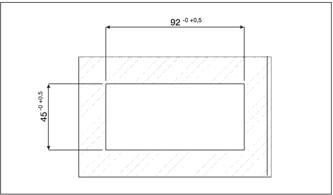
Panel cutout
