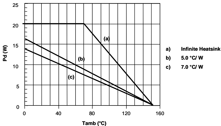
Figure 10. Power derating curve
