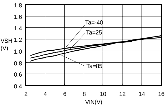
VSH-VIN S-8520/21
