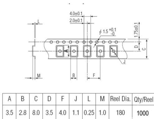
Figure 3) Pocket Tape Dimensions
