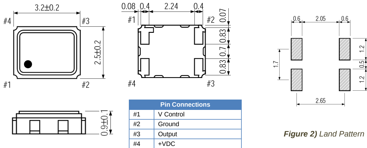
Figure 1) Top, Side, and Bottom views
