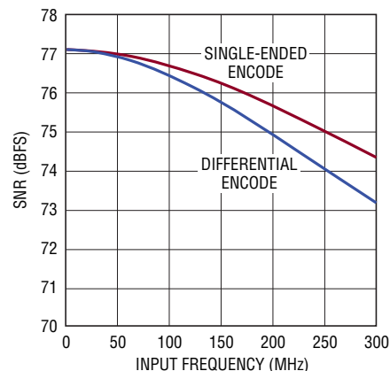
LTC2183: SNR vs Input Frequency, -1\text{dBFS} , 80\text{Mps} , 2\text{V} Range
