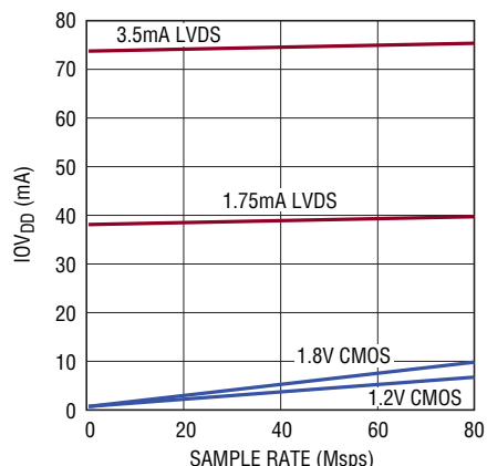
LTC2183: I_{OVPD} vs Sample Rate, 5\text{MHz} , -1\text{dBFS} Sine Wave Input on Each Channel
