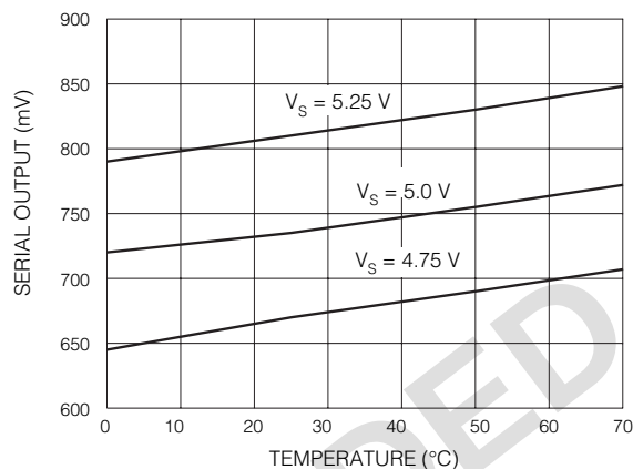
Fig. 4 Data and Data Output Voltage vs Temperature
