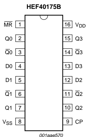
Fig 3. Pin configuration SOT38-4 and SOT109-1
