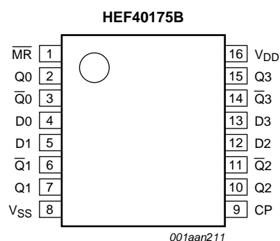
Fig 4. Pin configuration SOT403-1
