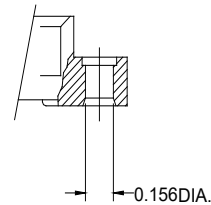
VARIATION 04 .156 +0.002 -0.000 DIA. MOUNTING HOLE
