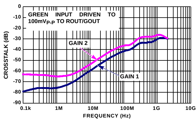
FIGURE 14. ACTIVE CHANNEL CROSSTALK
