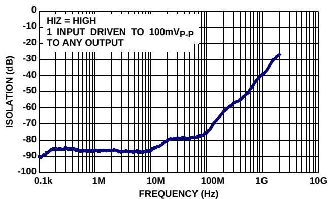
FIGURE 16. DISABLED ISOLATION
