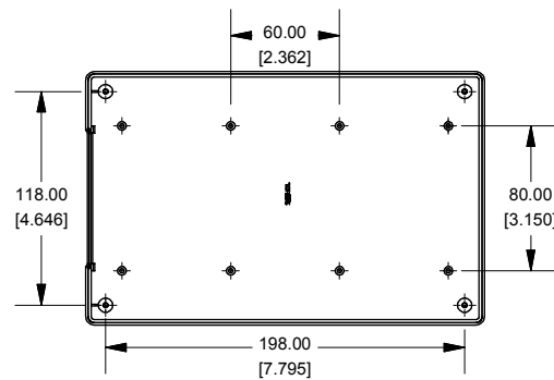
Bottom View Looking Inside Box
