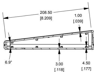
SECTION A-A Side View of Assembly
