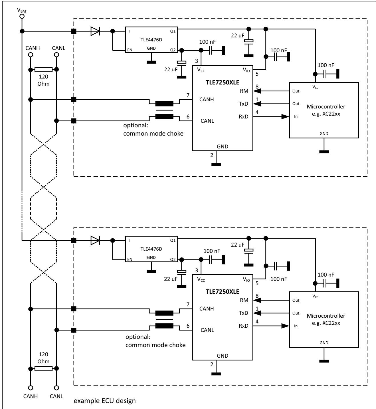
Figure 13 Application circuit
