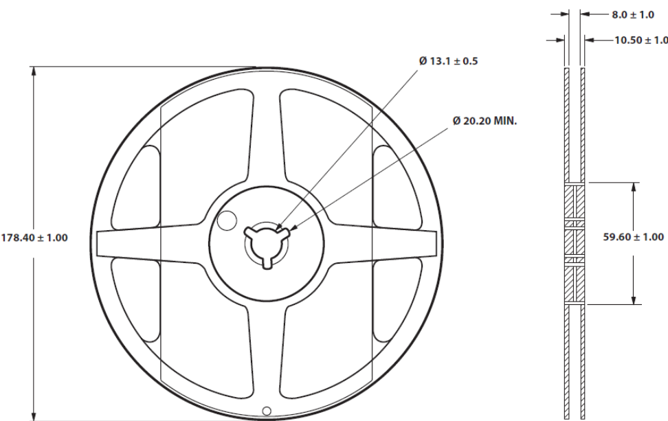
Figure 8: Reel Dimensions
