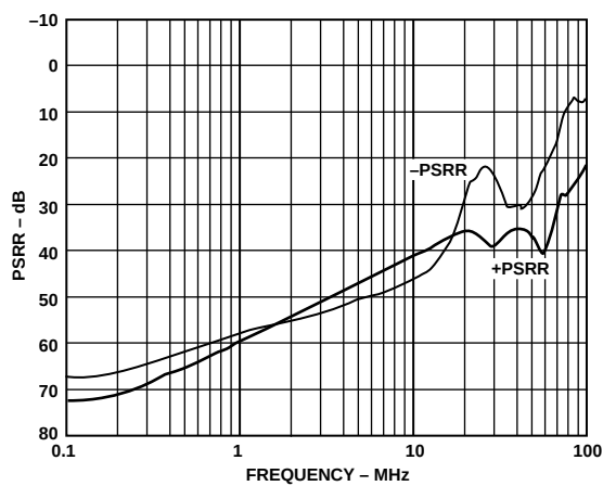
Figure 25. AD8185 PSRR vs. Frequency
