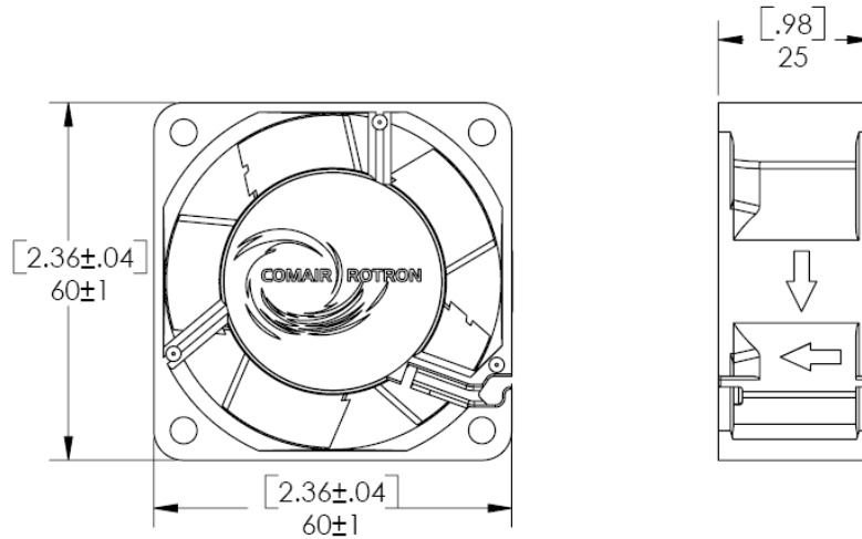
MECHANICAL DRAWING
