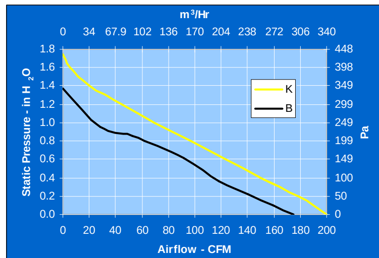
PERFORMANCE GRAPH
