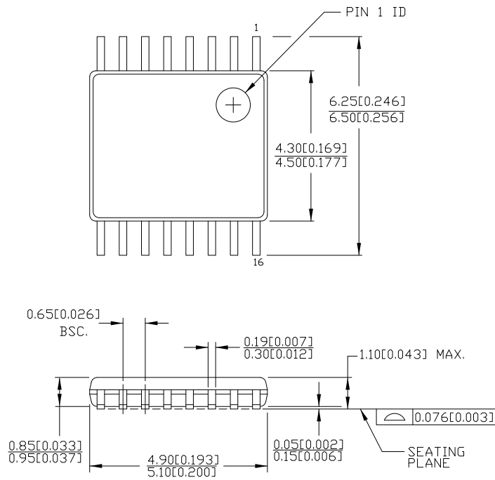
Figure 6. 16-pin TSSOP 4.40 mm Body Z16.173/ZZ16.173, 51-85091
