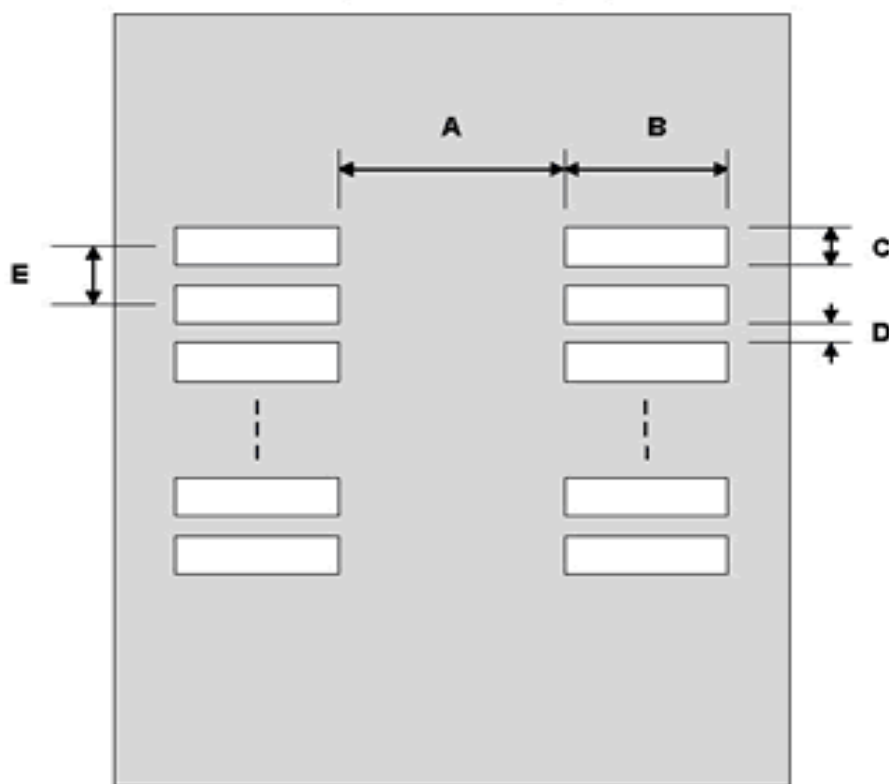
Top View (SMT Footprint)
