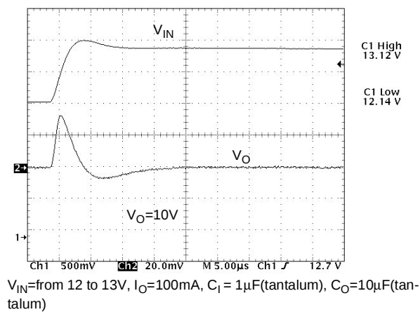
Figure 15 : Line Transient
