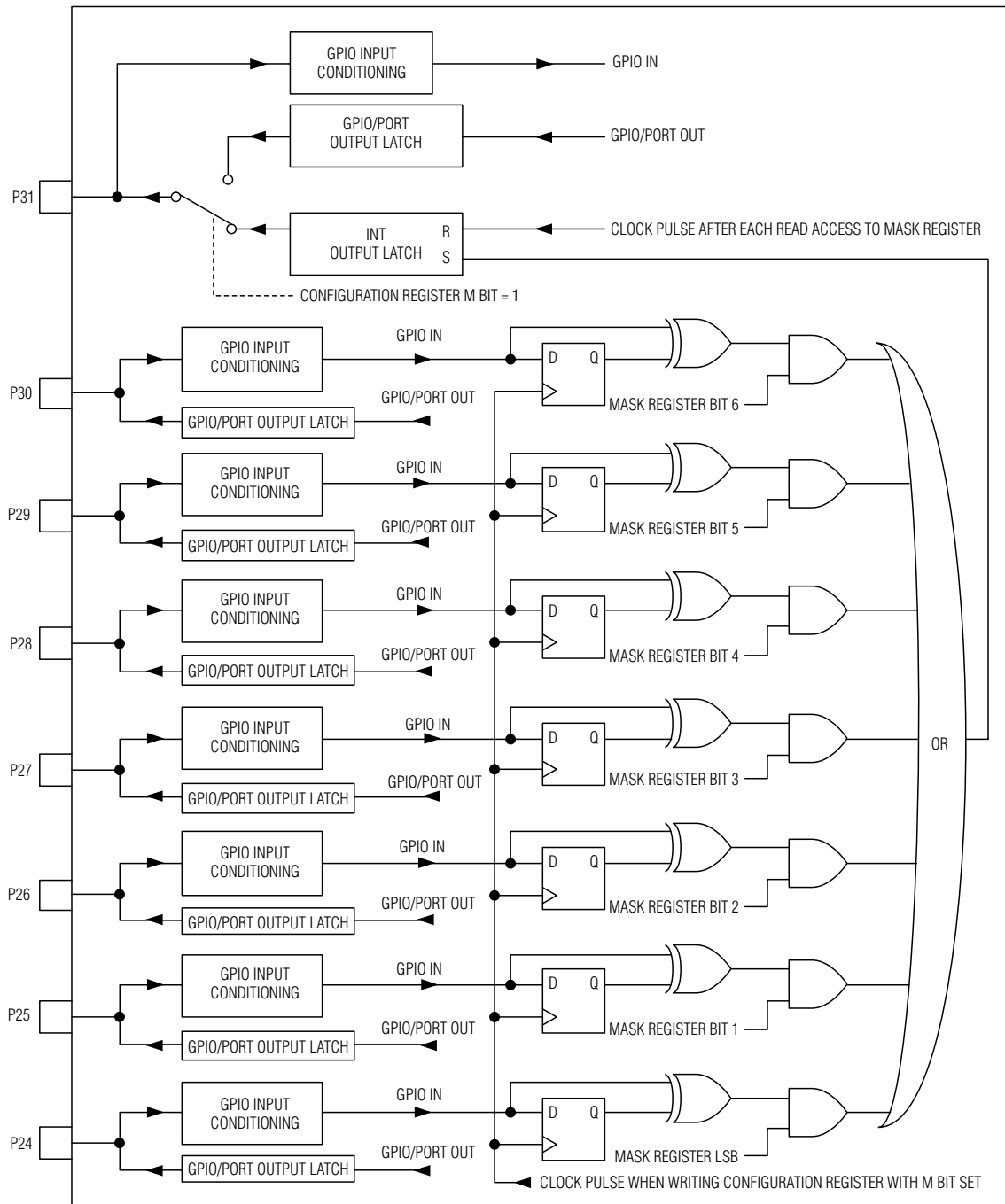
Figure 6. Maskable GPIO Ports P24 Through P31
