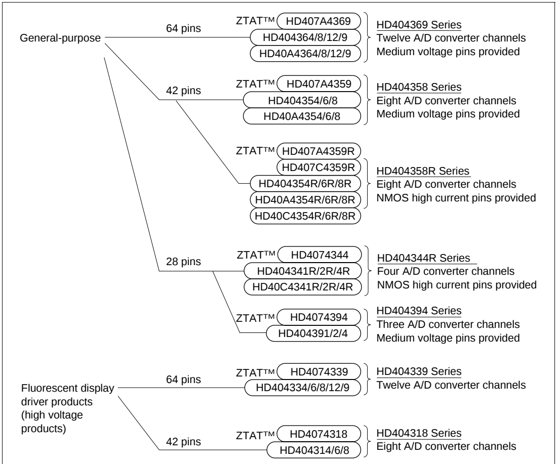
Figure 1-1 Structure of the HMCS43XX Family
