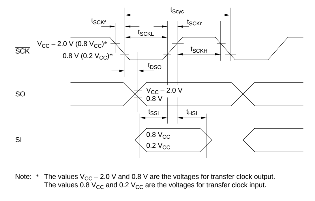
Figure 25-29 Serial Interface Timing (HD404339 Series)
