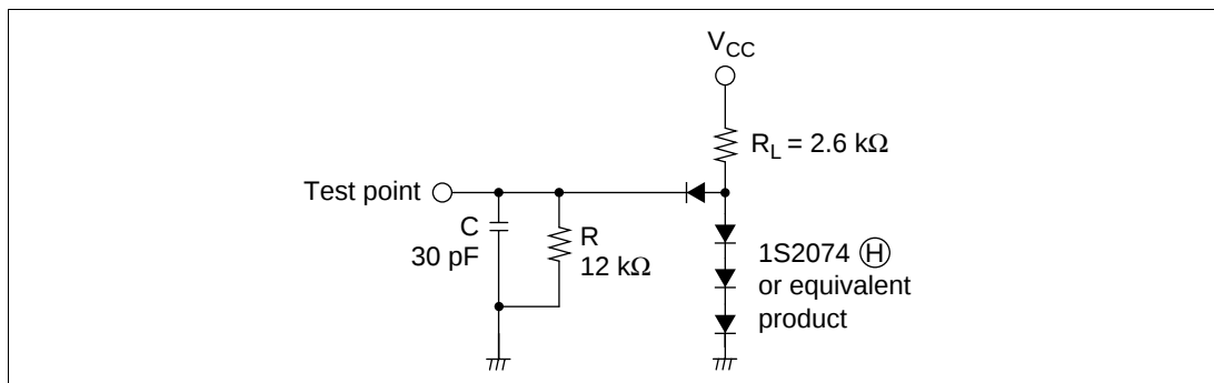
Figure 25-30 Timing Load Circuit
