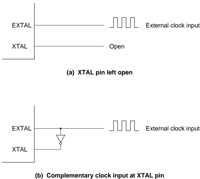
Figure 23.5 External Clock Input (Examples)
