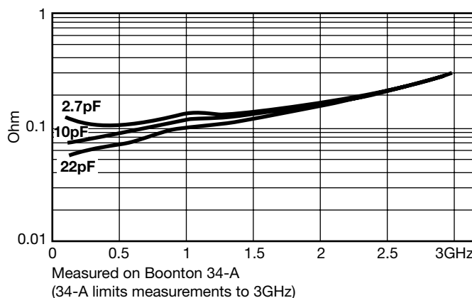
Typical ESR vs. Frequency Accu-F®/Accu-P® 0603
