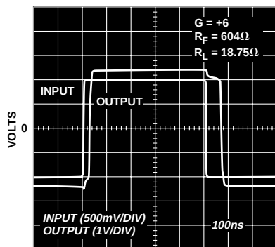
Figure 27. Overdrive Recovery; G = +6
