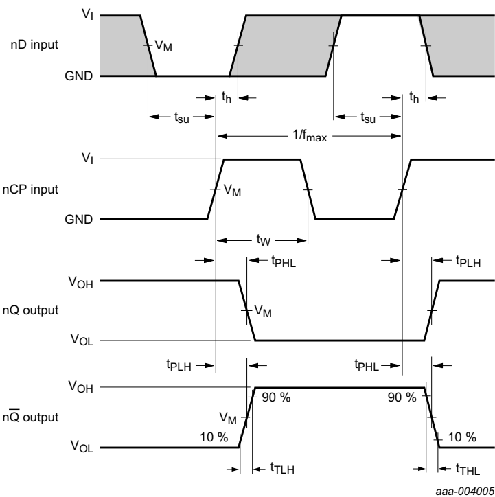
Measurement points are given in Table 9 . V_{OL} and V_{OH} are typical voltage output levels that occur with the output load. Fig 7. Input to output propagation delay, output transition time, clock input pulse width and maximum frequency
