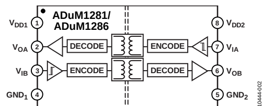
Figure 2. ADuM1281/ADuM1286
