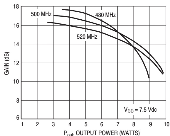
Figure 4. Gain versus Output Power
