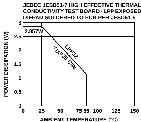
FIGURE 10. POWER DISSIPATION vs AMBIENT TEMPERATURE
