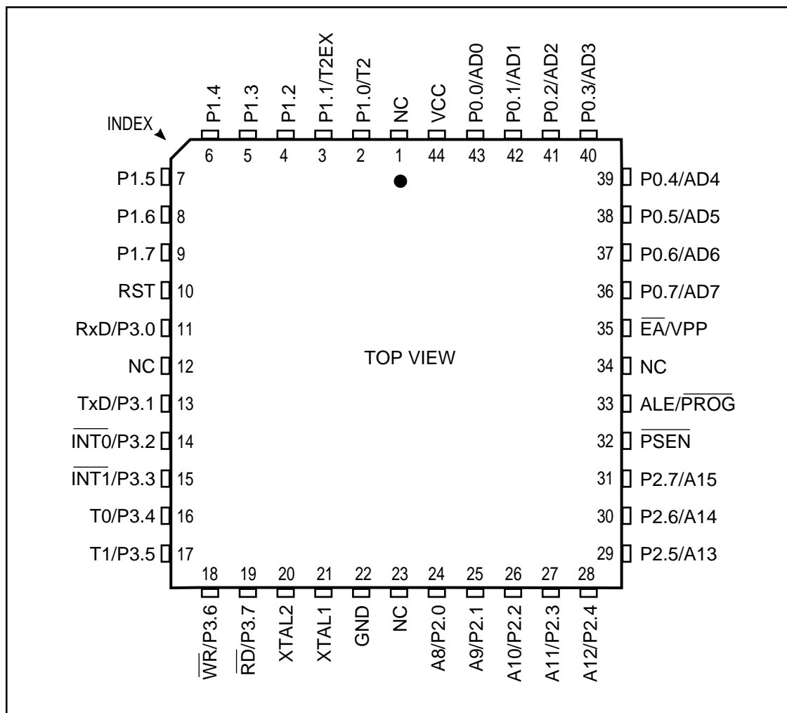
Figure 2. IS89C52 Pin Configuration: 44-pin PLCC
