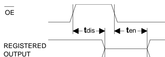
\overline{OE} to Output Enable/Disable
