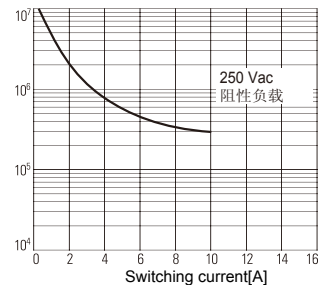
Electrical life
