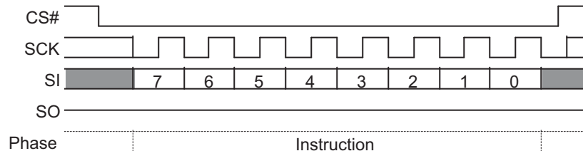
Figure 59. Write Enable (WREN 06h) Command Sequence
