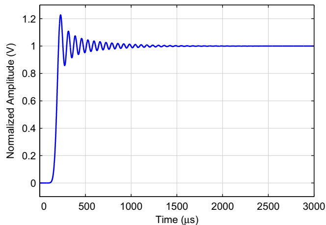
Figure 9-12. Step Response—Minimum Phase
