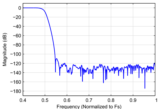
Figure 9-8. Stopband Attenuation
