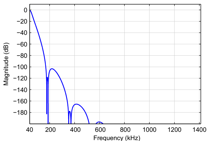
Figure 9-67. Stopband Attenuation
