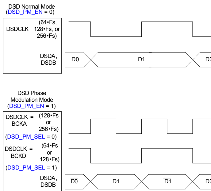
Figure 4-29. DSD Phase Modulation Mode Diagram
