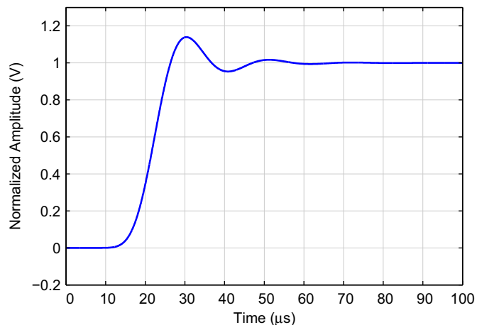
Figure 9-69. Step Response
