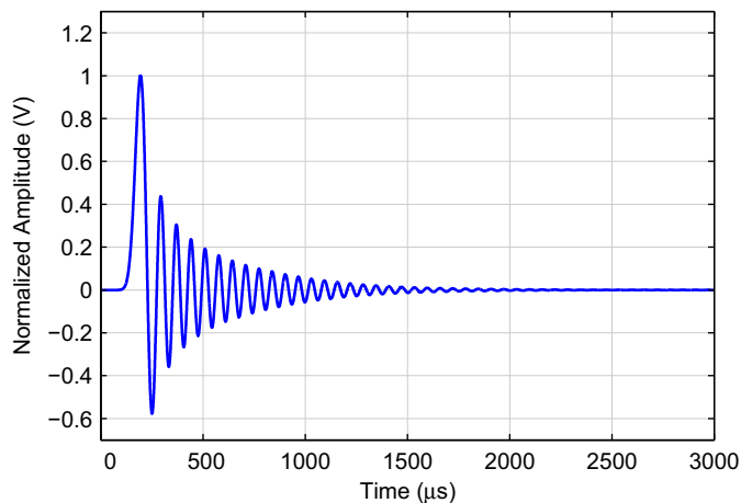
Figure 9-10. Impulse Response—Minimum Phase
