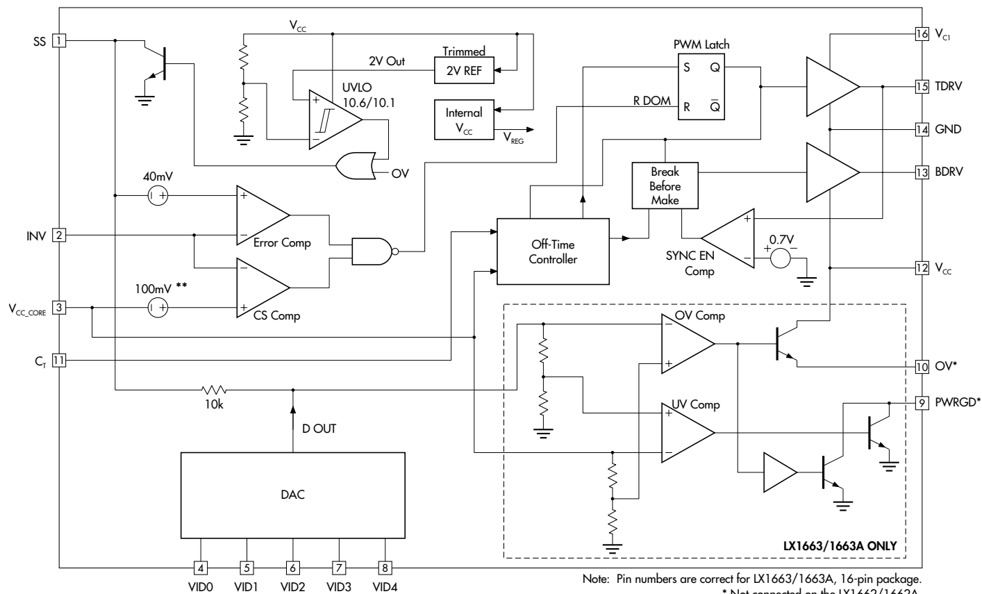
FIGURE 5 — Block Diagram
