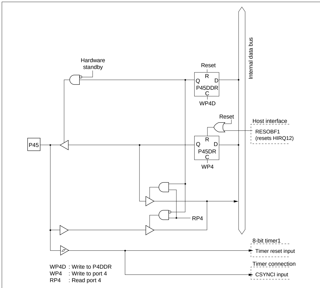
Figure C.13 Port 4 Block Diagram (Pin P45)
