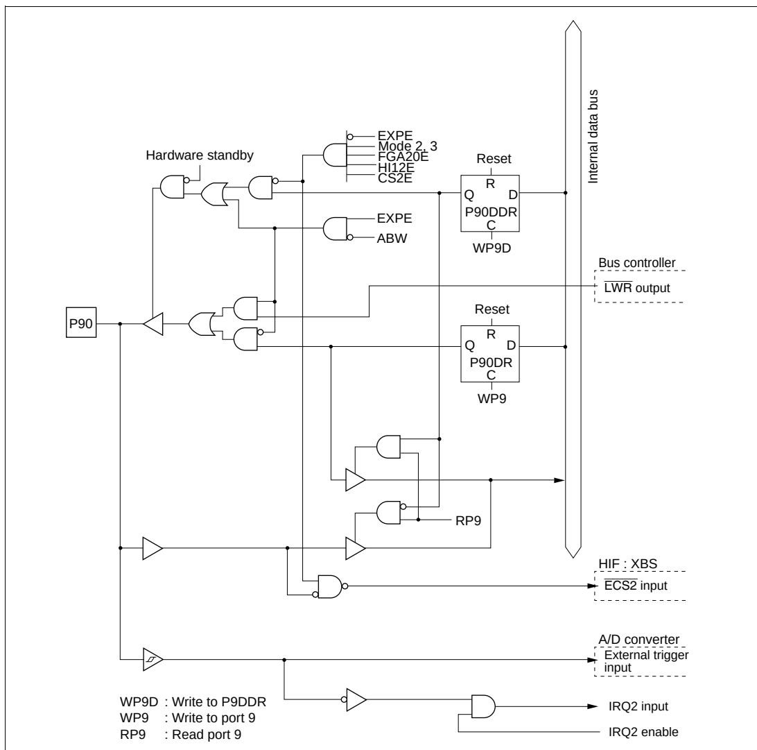
Figure C.32 Port 9 Block Diagram (Pin P90)
