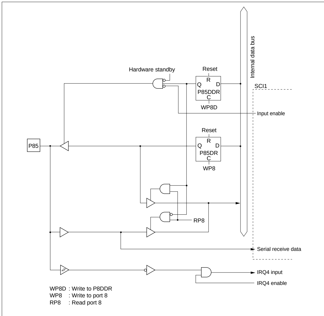
Figure C.30 Port 8 Block Diagram (Pin P85)
