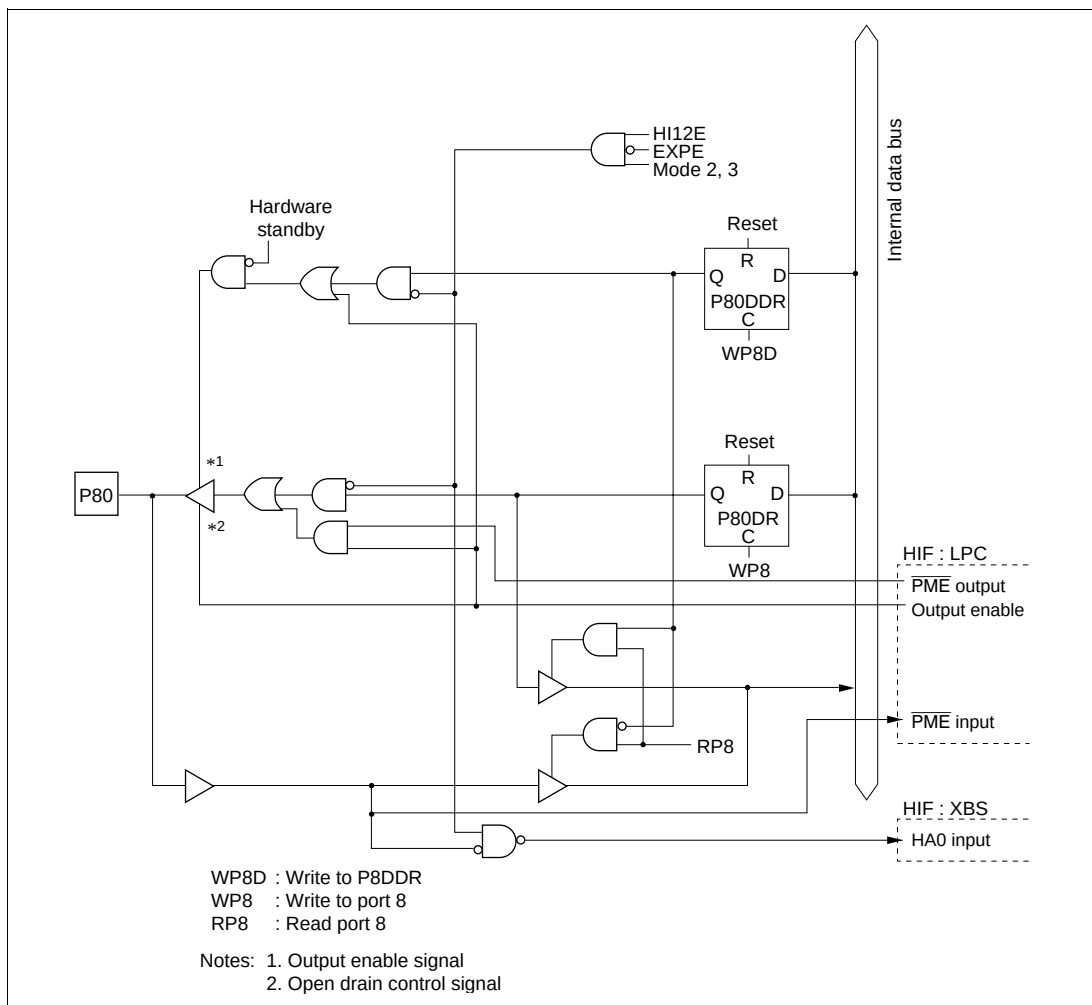
Figure C.25 Port 8 Block Diagram (Pin P80)
