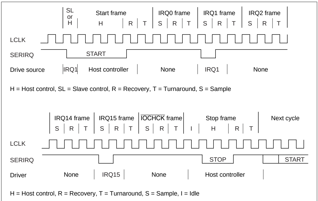
Figure 18B.6 SERIRQ Timing
