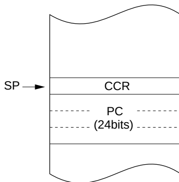
Figure 4.5 (1) Stack Status after Exception Handling (Normal Mode)
