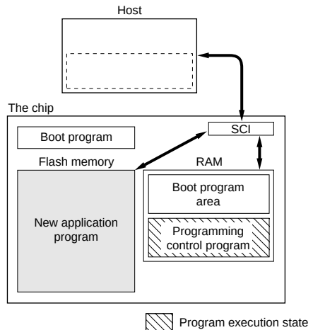
Figure 22.4 Boot Mode
