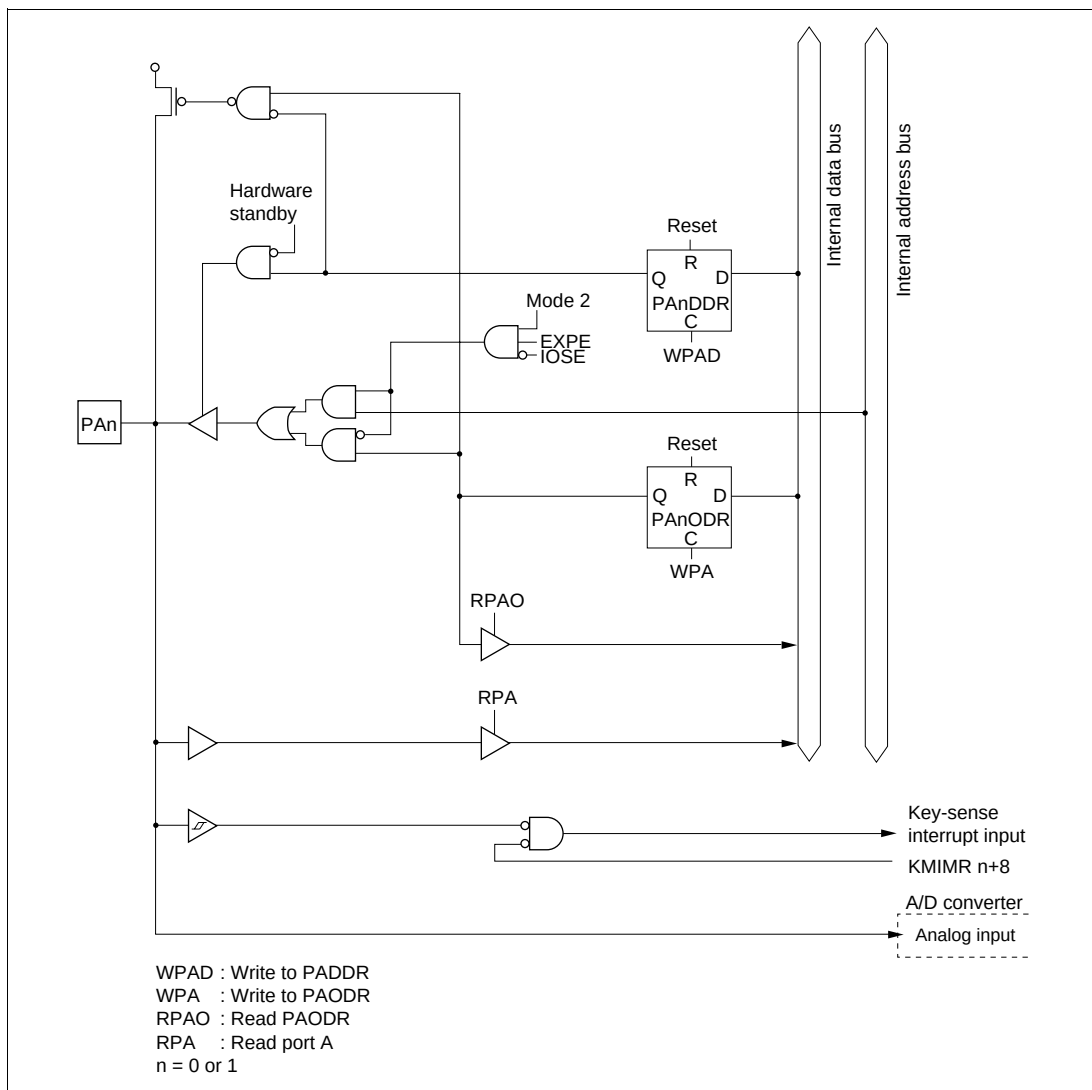
Figure C.37 Port A Block Diagram (Pins PA0, PA1)
