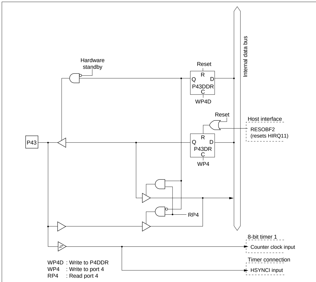
Figure C.11 Port 4 Block Diagram (Pin P43)
