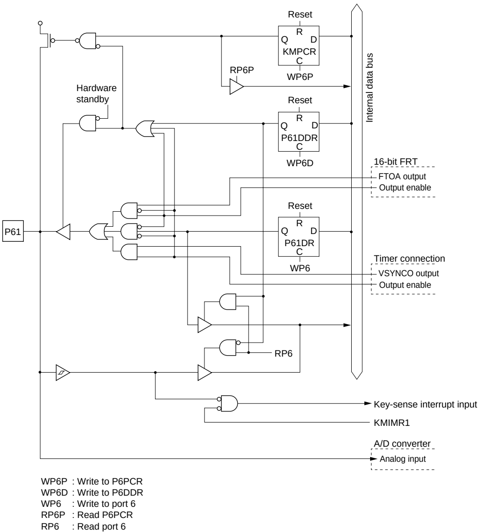
Figure C.19 Port 6 Block Diagram (Pin P61)
