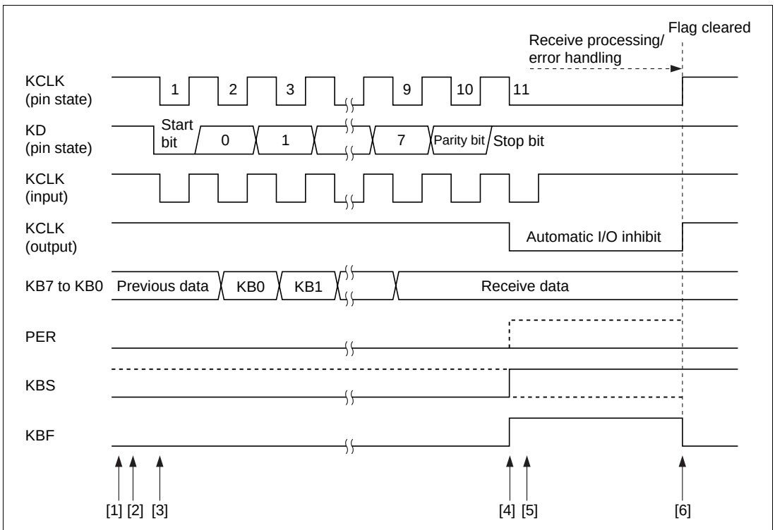
Figure 17.4 Receive Timing
