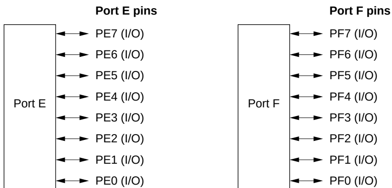
Figure 8.21 Pin Functions for Ports E and F
