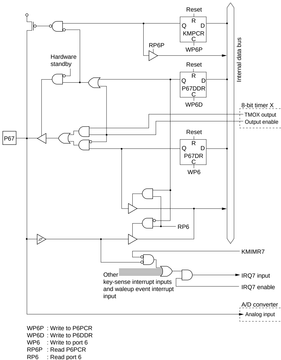
Figure C.22 Port 6 Block Diagram (Pin P67)
