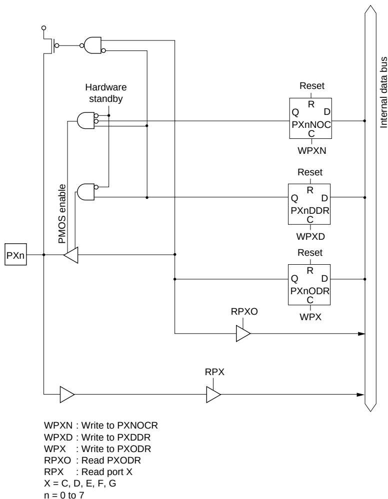
Figure C.43 Port C, D, E, F, G Block Diagram
