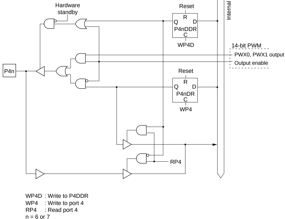
Figure C.14 Port 4 Block Diagram (Pins P46, P47)
