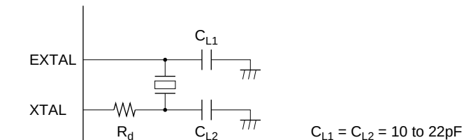
Figure 23.2 Connection of Crystal Resonator (Example)
