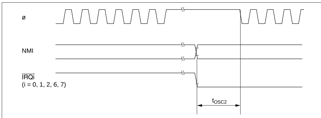
Figure 25.6 Oscillation Settling Timing (Exiting Software Standby Mode)
