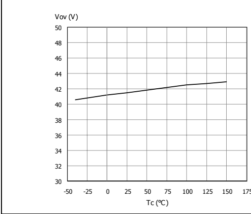
Figure 11. Over-voltage shutdown
