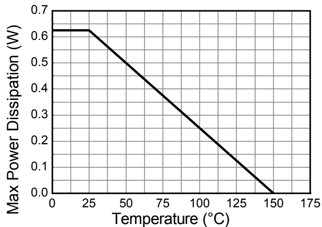
Derating Curve
