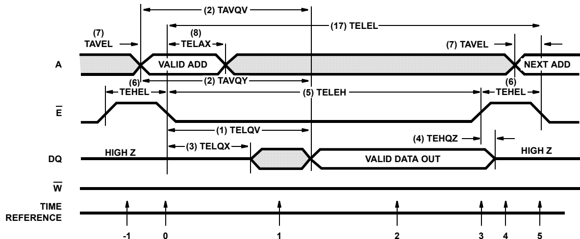
FIGURE 1. READ CYCLE
