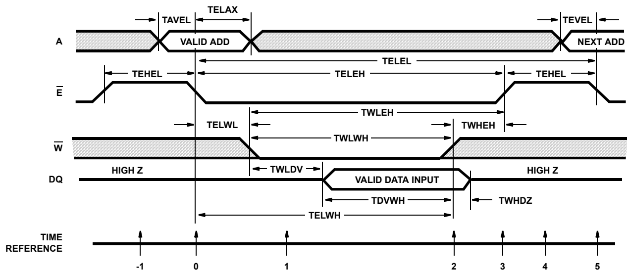
FIGURE 2. WRITE CYCLE
