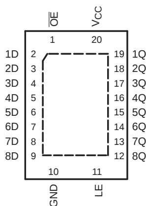
SN74LVC573A . . . RGY PACKAGE (TOP VIEW)
