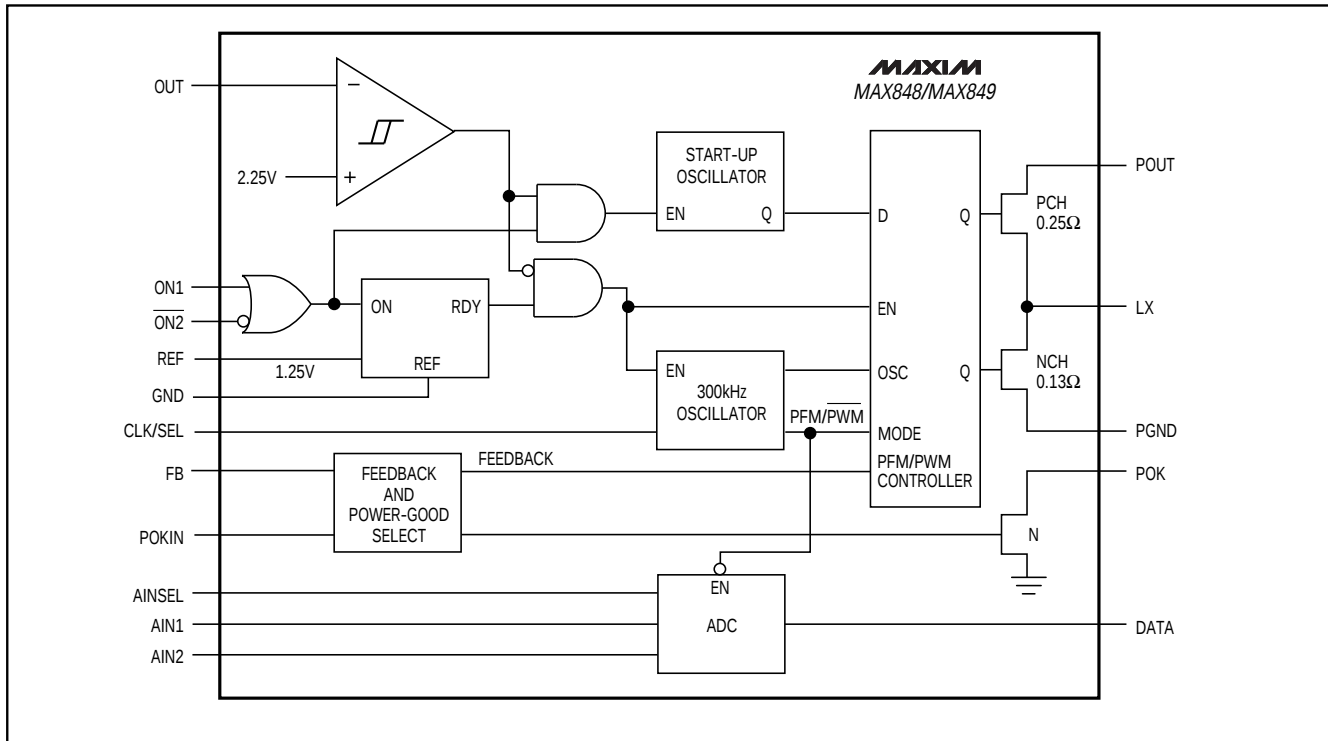
Figure 1. Functional Diagram
