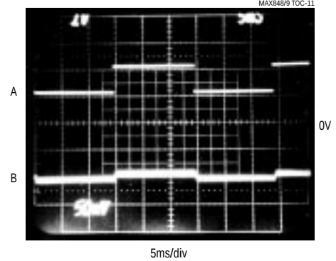
LINE-TRANSIENT RESPONSE
