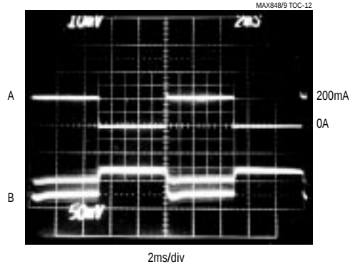
LOAD-TRANSIENT RESPONSE
