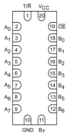
Pin Assignment for DQFN
