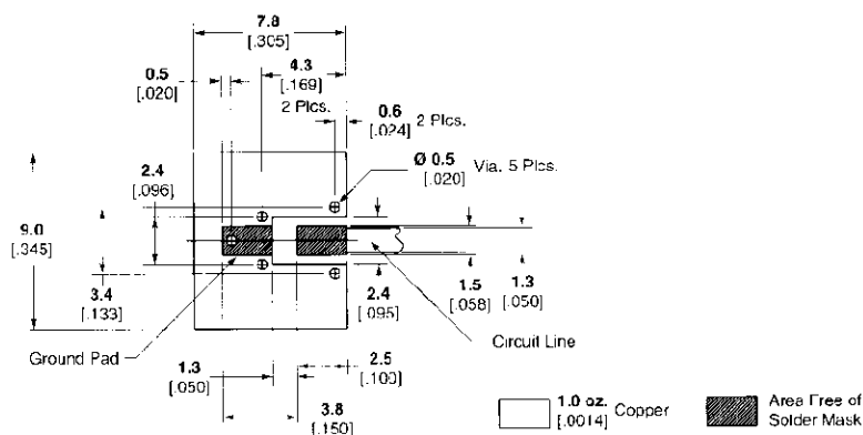
Recommended Mounting Pattern for Microstrip Line
