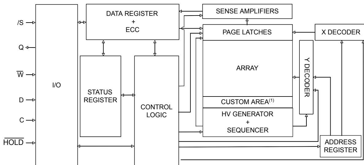
Figure 3. Block diagram
