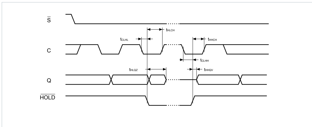
Figure 20. Hold timing
