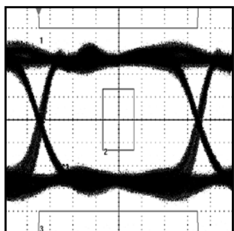
OPTICAL EYE DIAGRAM ( I_{MOD} = 40\text{mA} , DATA RATE = 2.56Gbps, PATTERN 213 - 1 + 80CID)
