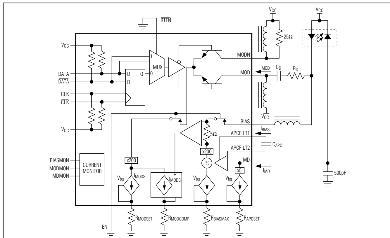
Figure 3. Functional Diagram
