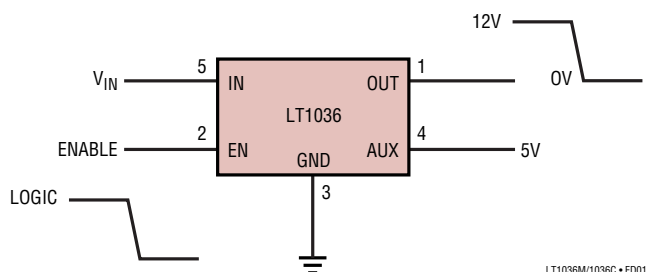
Functional Diagram
