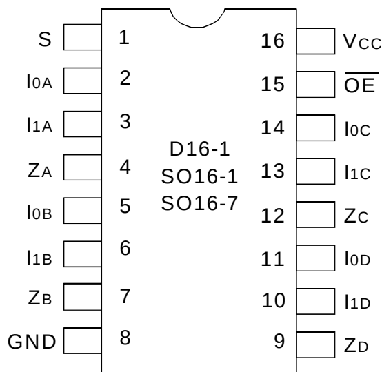
CERDIP/ SOIC/ QSOP/ CERPACK TOP VIEW
