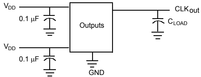
Figure 2. Test Circuit
