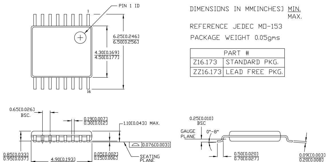
Figure 8. 16-pin TSSOP 4.40 mm Body Z16.173/ZZ16.173 Package Outline, 51-85091
