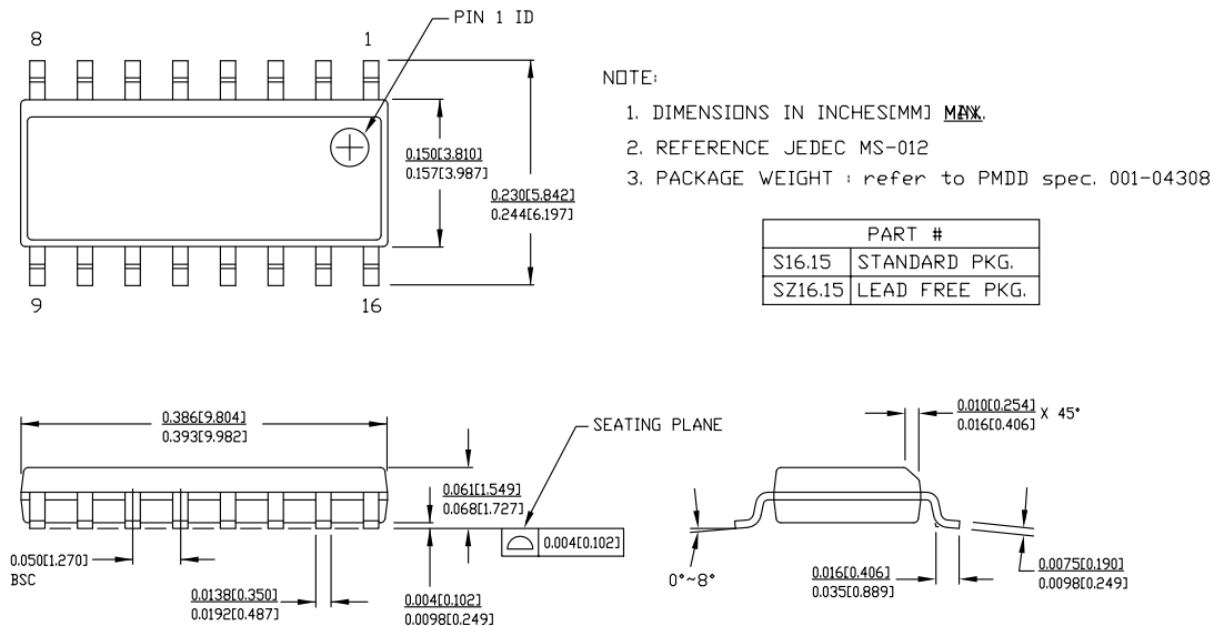
Figure 7. 16-pin SOIC (150 Mils) S16.15/SZ16.15 Package Outline, 51-85068
