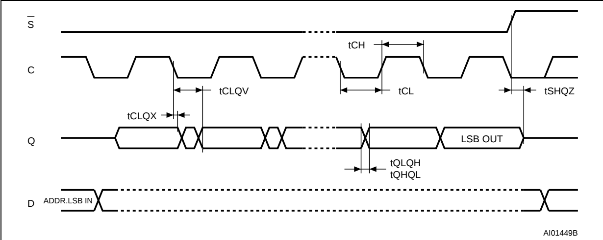
Figure 16. Output Timing
