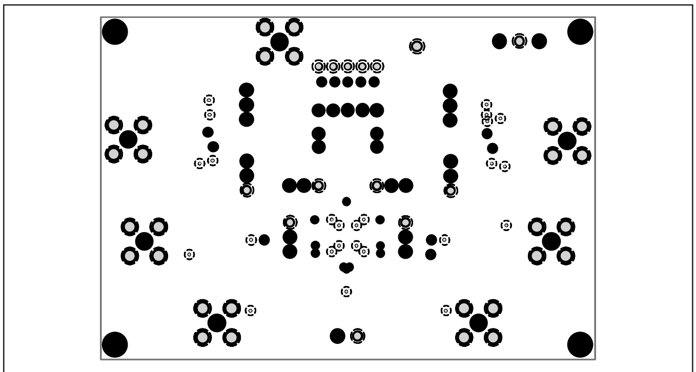
FIGURE 3. Ground Layer.
