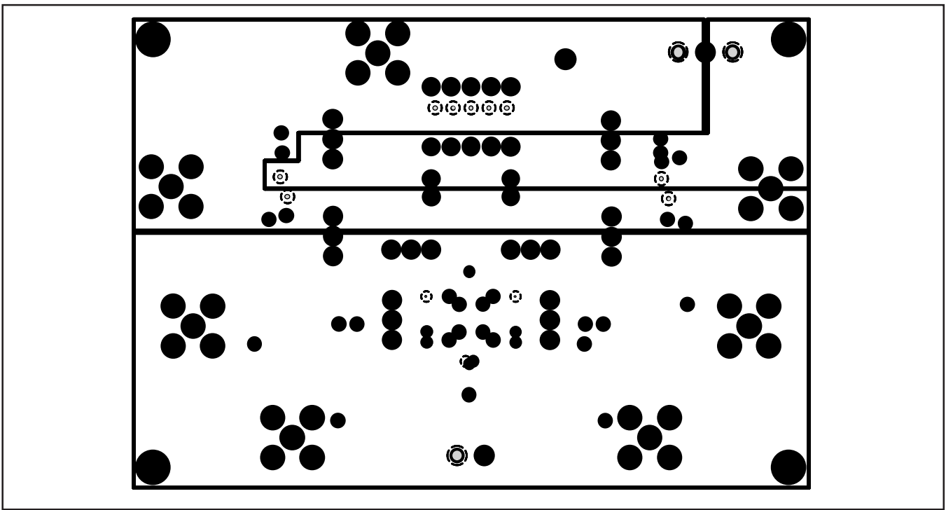
FIGURE 4. Power Layer.
