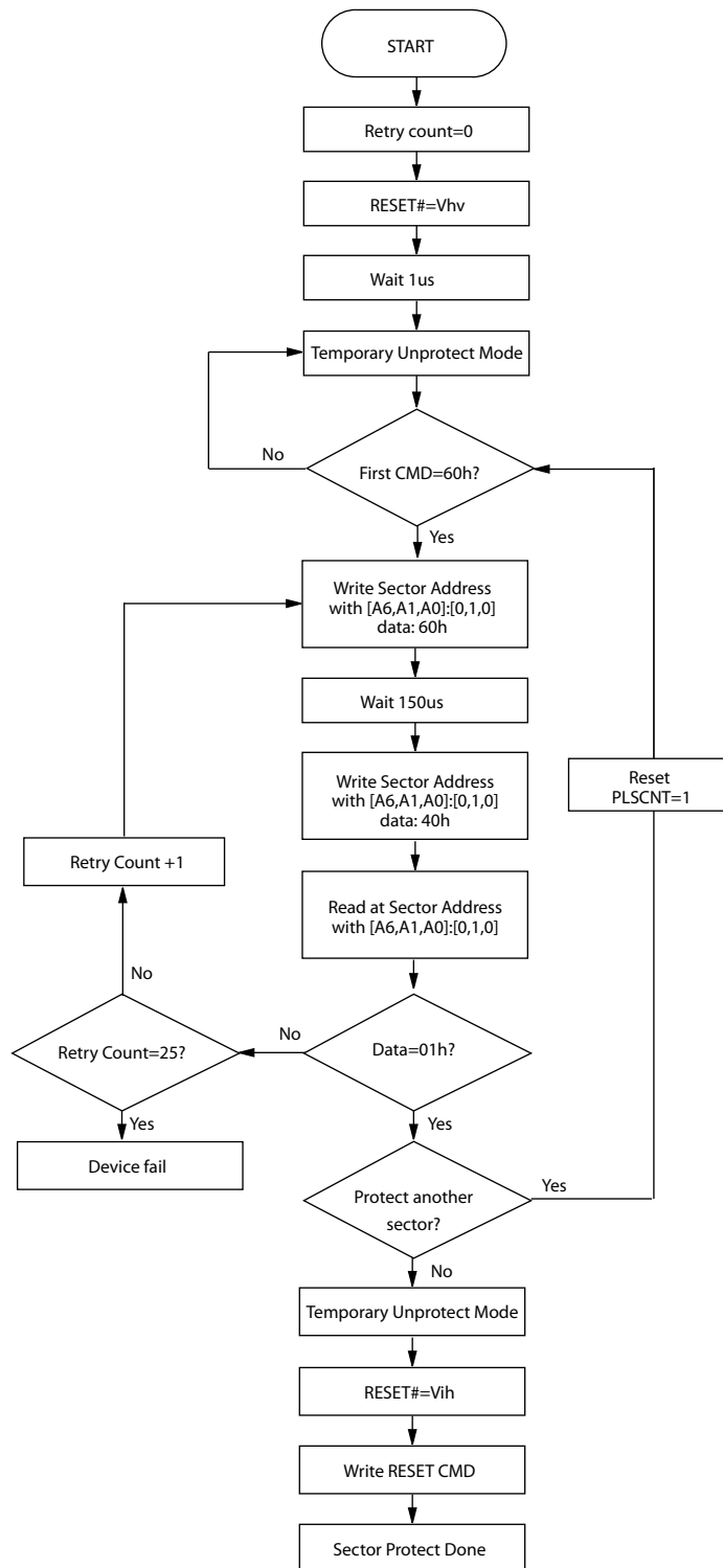
Figure 13-1. IN-SYSTEM SECTOR PROTECT WITH RESET#=Vhv
